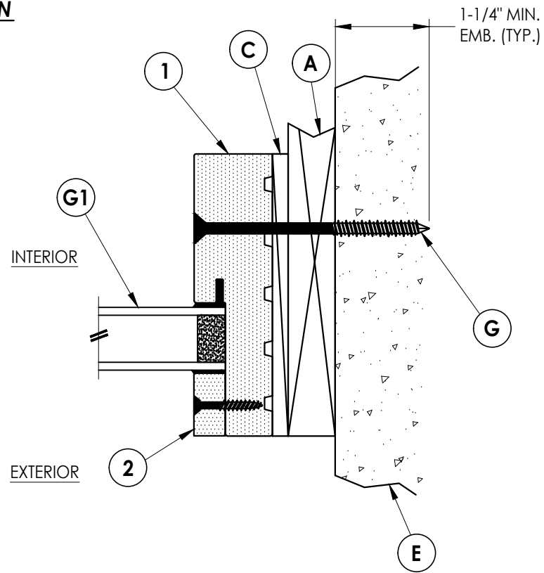
2 2 HORIZONTAL CROSS SECTION Shown w/ 1X buck
